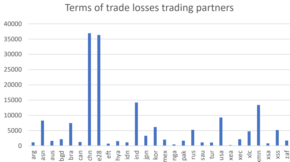
Figure A1: Terms of trade spillovers: terms of trade losses trading partners because of actual tariffs in comparison to zero tariffs
