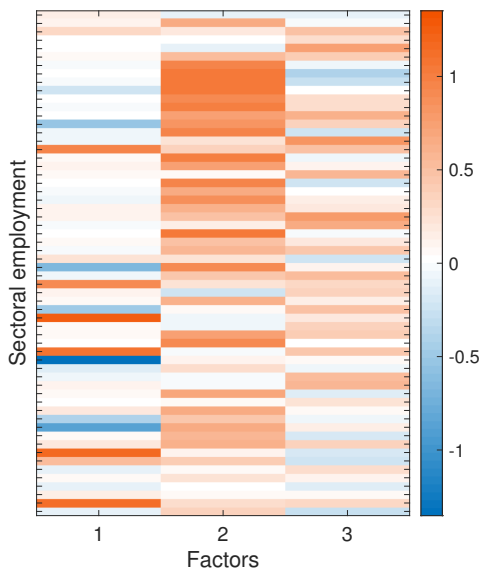
(a) Mean loadings
