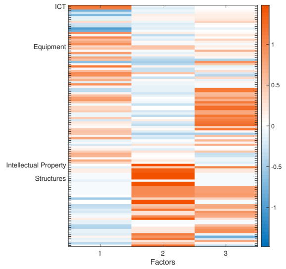
(b) Mean loadings
