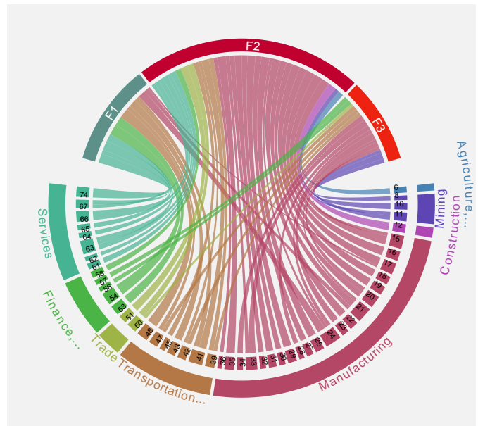
(b) Circos for non-zero loadings (95% HPDI)
