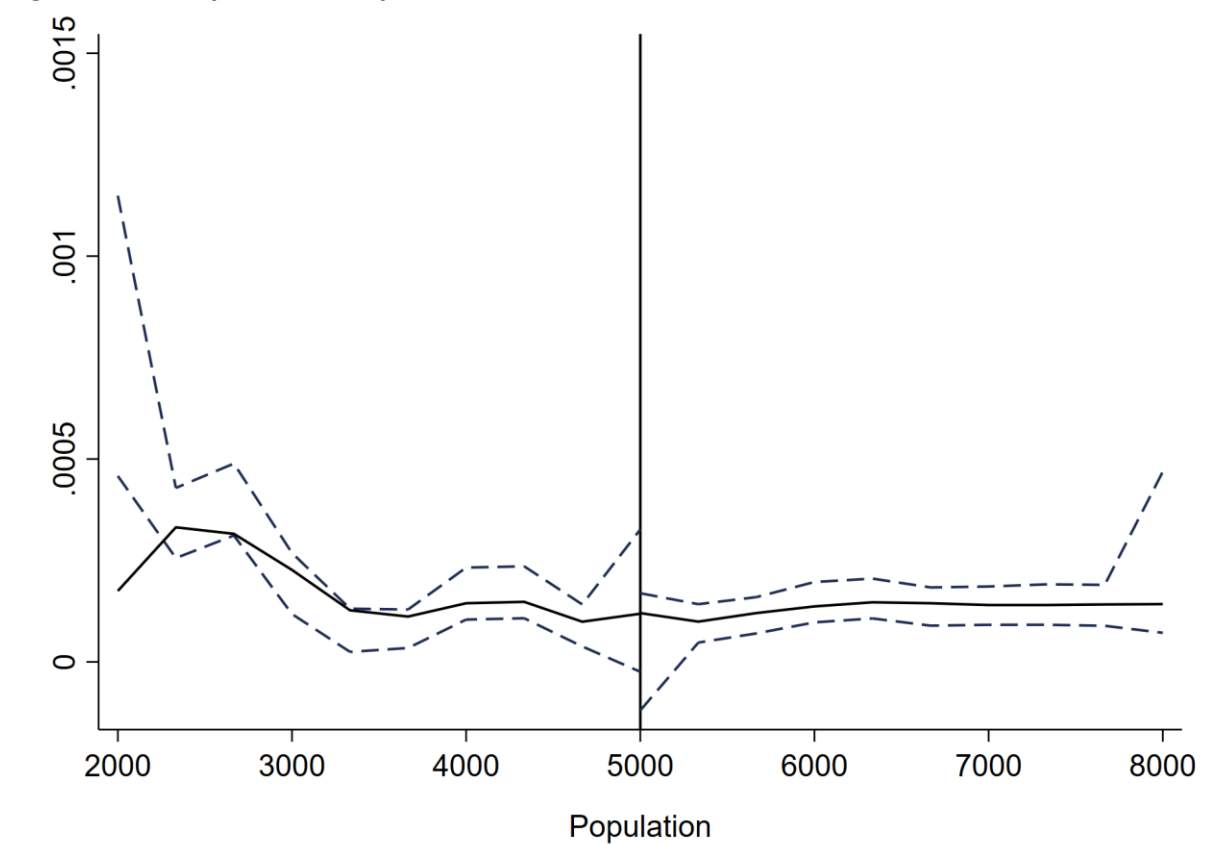
Figure 1: McCrary test – density around the 5,000 inhabitant threshold
