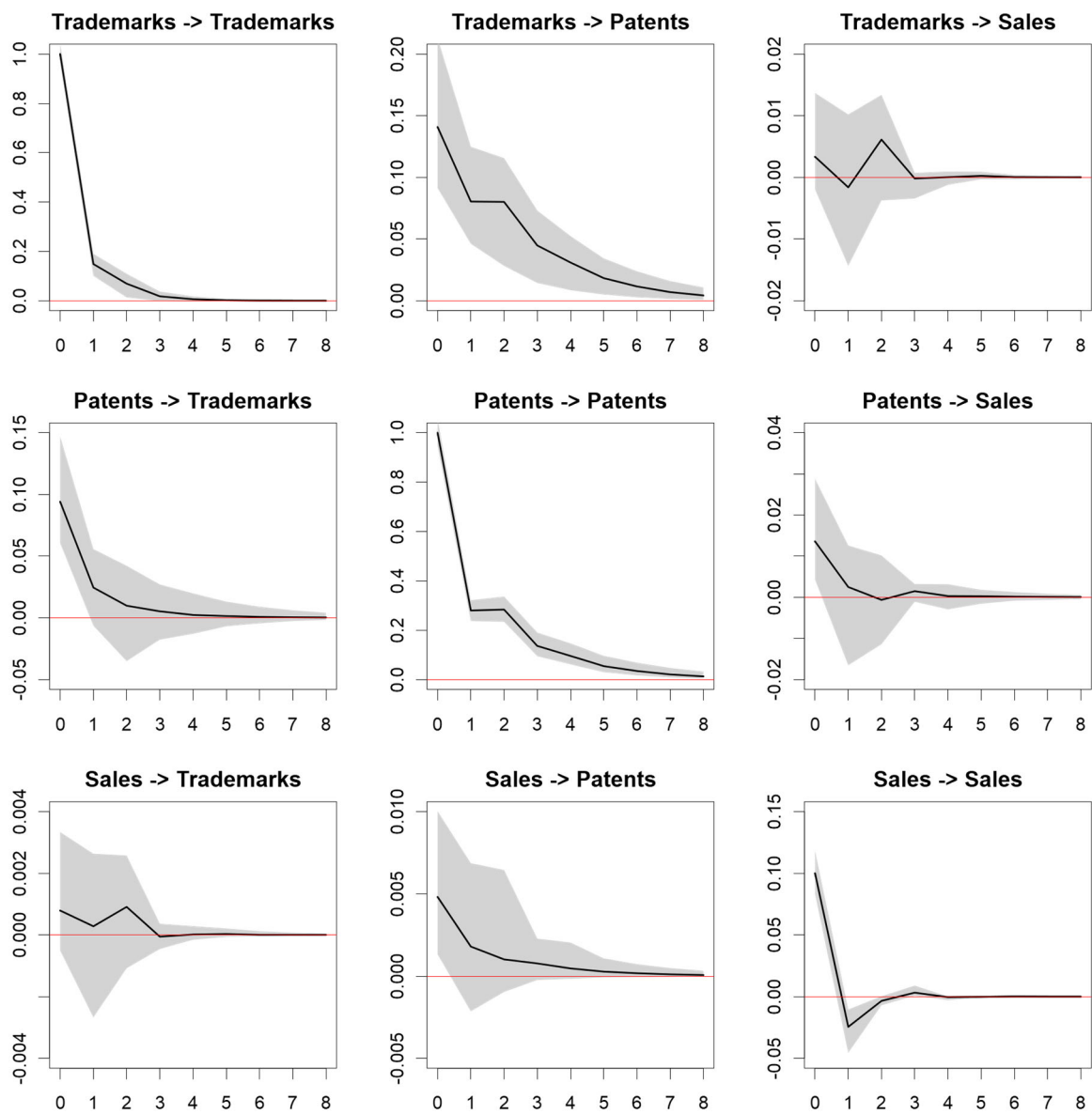
Fig. 1 Impulse Responses for Baseline Specification (Imputed Dataset)
