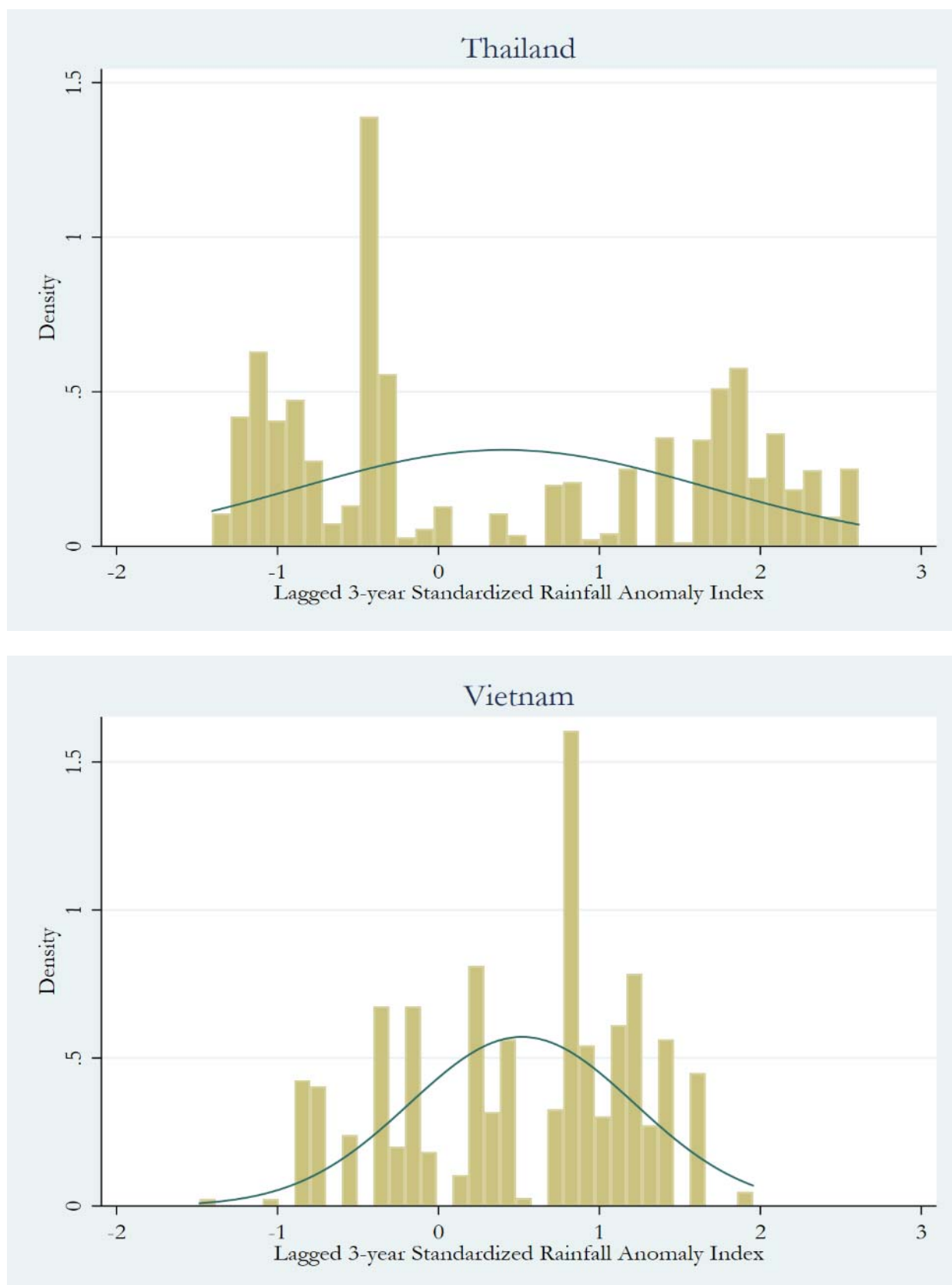
Figure A1. Distribution of the lagged Standardized Rainfall Anomaly Index in Thailand and Vietnam for the year of 2013 and 2016
