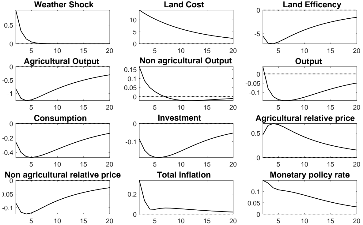
Figure 5: IRF to a one Celsius degree shock in the ENSO index.
