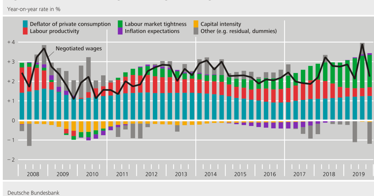
Figure 6: Contributions to the growth of negotiated wages
