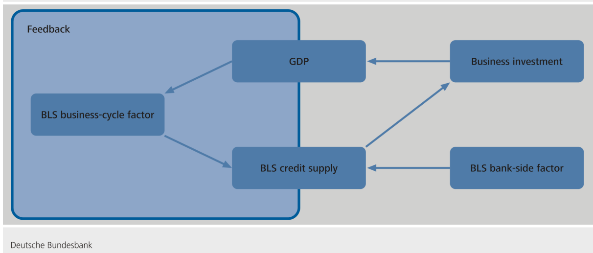
Figure 2: Macro-financial feedback mechanism in BbkM-DE
