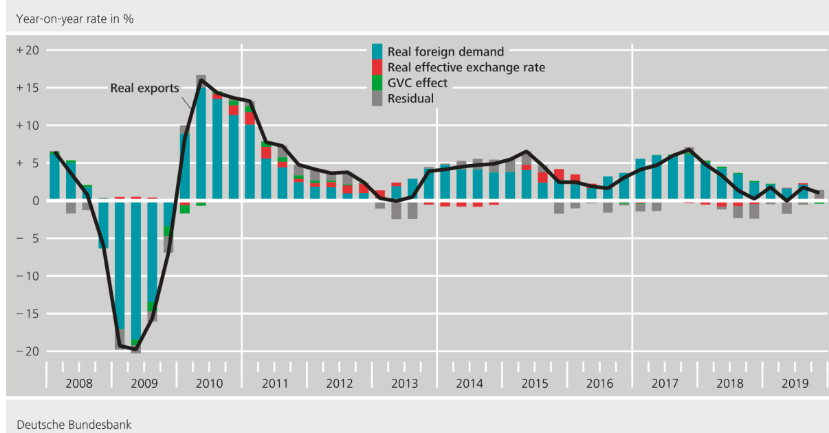
Figure 5: Contributions to real export growth
