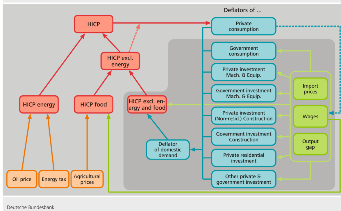
Figure 3: Structure of the domestic price block in BbkM-DE
