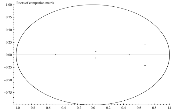
Figure 2: Roots of the system with common shifts. The system is restricted to have equal intercepts before 1974 and after 1996, as described before. The fact that the moduli of the roots are clearly smaller than unity implies that the series are I(0) with breaks, not I(1) .
