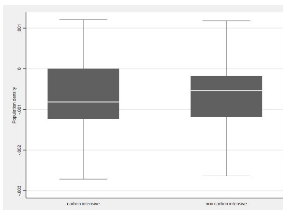
Figure 8 / Distribution of regression coefficients between carbon-intensive and non-carbon-intensive regions –population density and GDP
