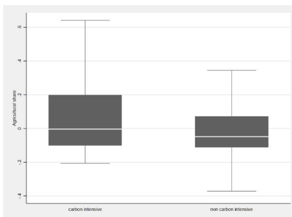
Figure 6 / Distribution of regression coefficients between carbon-intensive and non-carbon-intensive regions – employment growth and agricultural share
