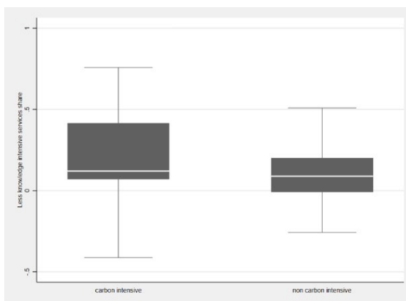
Figure 7 / Distribution of regression coefficients between carbon-intensive and non-carbon-intensive regions –industry and services share
