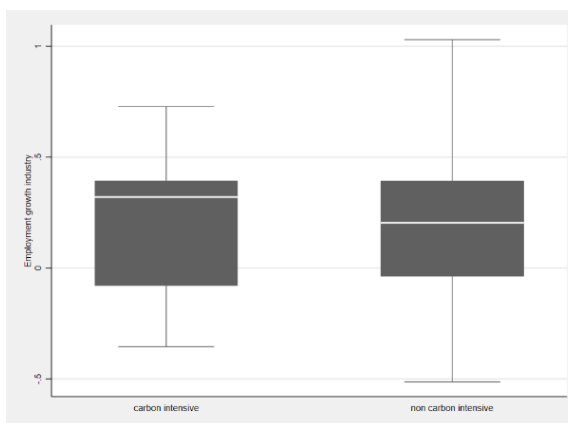
Figure 10 / Distribution of regression coefficients between carbon-intensive and non-carbon-intensive regions –employment growth in agriculture and industry
