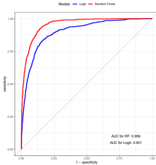
Figure 3: ROC curve for top 1 percent of wealth (RFs vs. logits)
