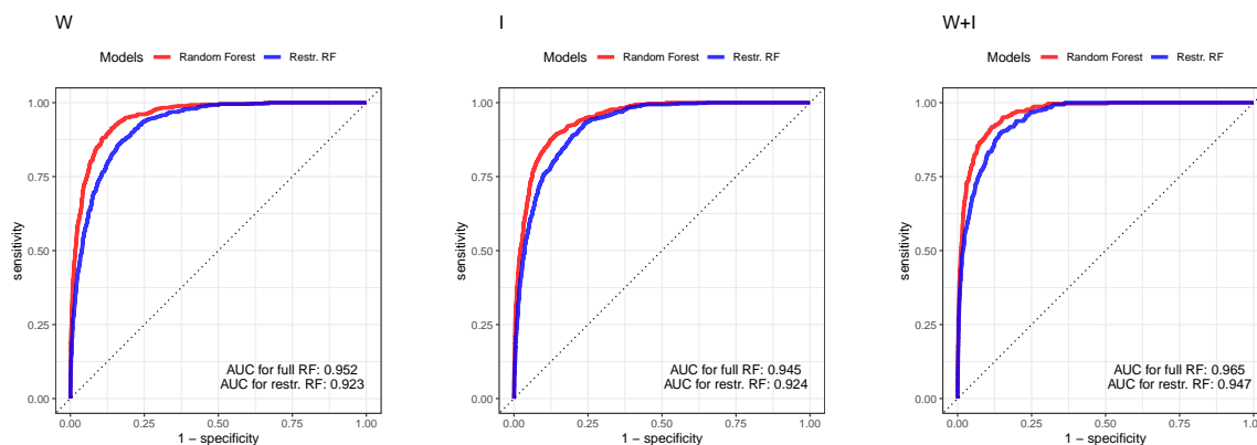
Figure 8: Restricted Random Forests: ROC curves for top 1 percent groups
