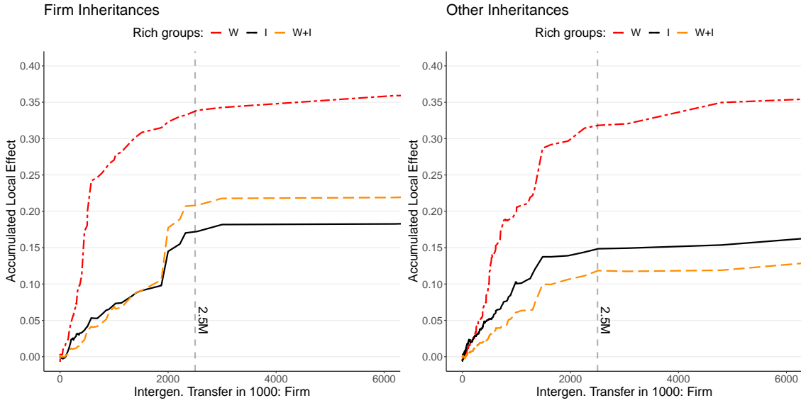
Figure 7: Accumulated local effects for top 1 percent: Inheritances
