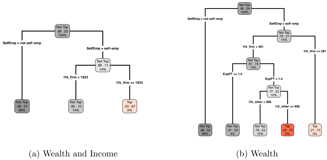
Figure 2: Single optimally pruned classification trees for top 1 percent group membership
