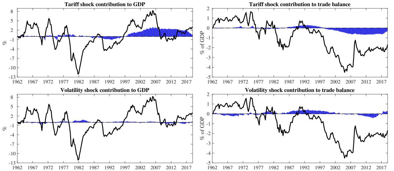
Figure 9: Historical decomposition of GDP and trade balance. Notes: The black lines show detrended data and the blue bars show the historical contribution of tariff level shocks (upper panels) and of trade policy uncertainty shocks (lower panels) to GDP (left panels) and to the trade balance (right panels). The trade balance is defined as net exports relative to GDP and is added in growth rates as an additional variable to the baseline model.
