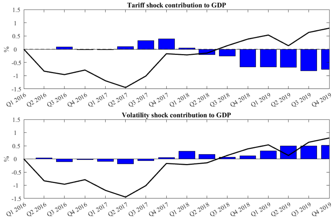
Figure A.7: Historical decomposition of output 2016Q1-2019Q4. Notes: Thick back lines show actual detrended data, thin blue lines show counterfactuals driven by the respective shock only.
