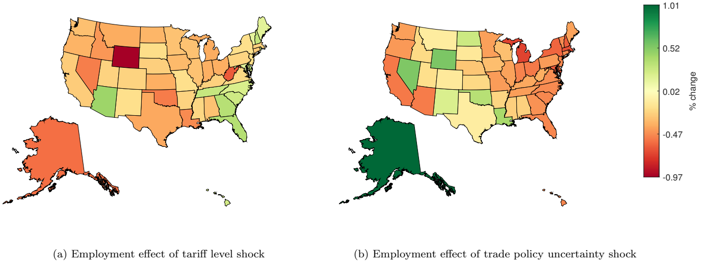
Figure 12: Peak employment effect across US states. Notes: The figure shows the absolute maximum response of state employment to a unit positive tariff level shock in panel (a) and to a unit positive trade policy uncertainty shock in panel (b), obtained from local projections. The colors indicate the sign and size of the effect.
