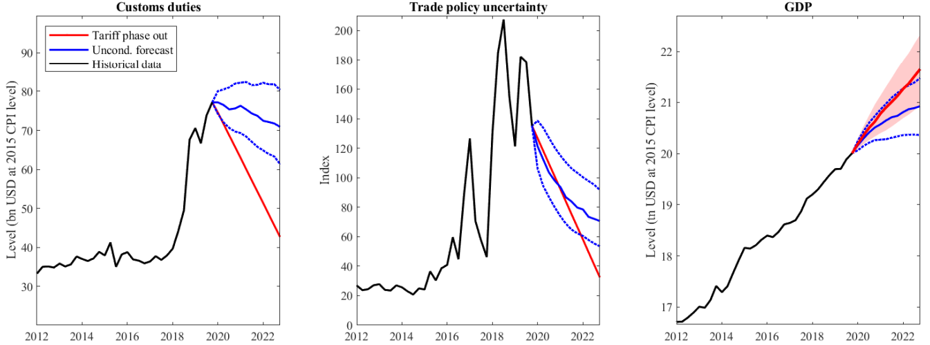
Figure 13: Structural scenario of return to free trade. Notes: The red solid line and shaded region in the third panel are the median forecast and 40% point-wise credible sets of GDP for a scenario in which customs duties and trade policy uncertainty revert to pre-2016 levels, shown by the red solid lines in the first two panels. The scenario is driven by trade policy level and uncertainty shocks. The blue dotted lines show medians and 40% point-wise credible sets of the unconditional forecasts of the model.
