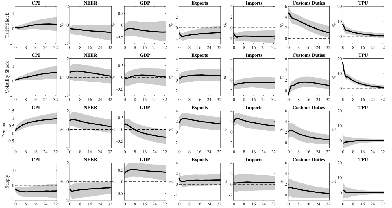
Figure A.4: Impulse responses to all four types of shocks. Notes: The figure shows the structural impulse responses to a tariff level shock, a trade policy uncertainty shock, a domestic demand shock, and a domestic supply shock in rows on the endogenous variables in columns. It reports point-wise median impulse responses and 68% highest posterior density credible sets.
