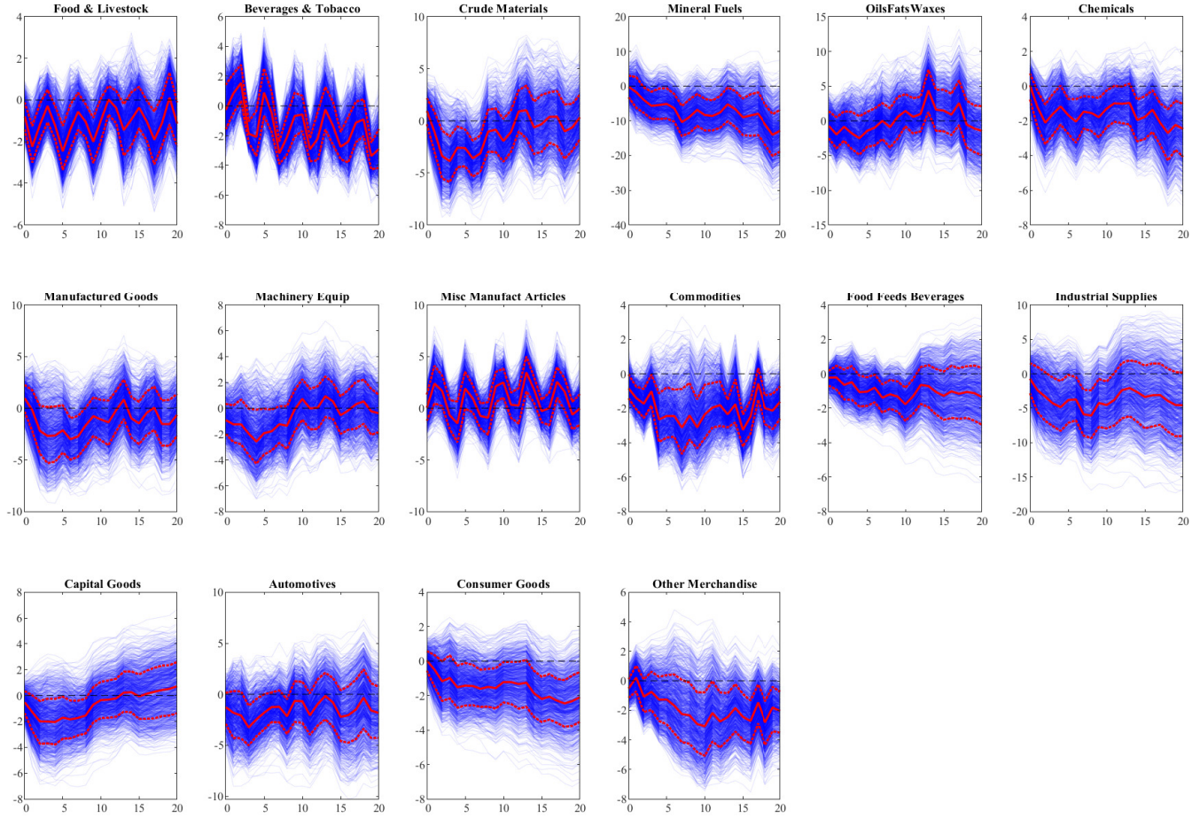
Figure A.11: Responses of sectoral imports to a tariff level shock. Notes: The figure shows the responses of sectoral imports obtained from local projections. It shows the responses for each of the 1000 draws and the point-wise median and 68% highest posterior density sets.
