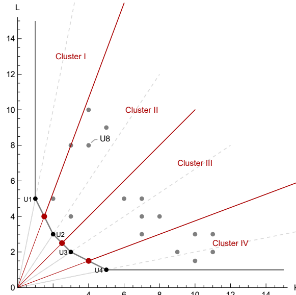
Fig. 1. Non-parametric-clustering approach
