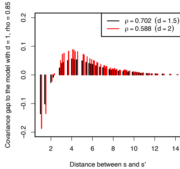
Figure 2: Numerical examples: interaction between \rho and d .
