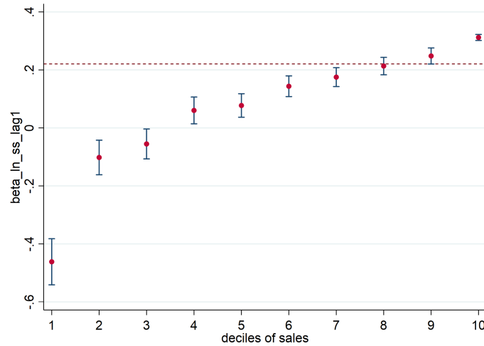
Figure 7: Heterogeneity by size, IV shift-share
