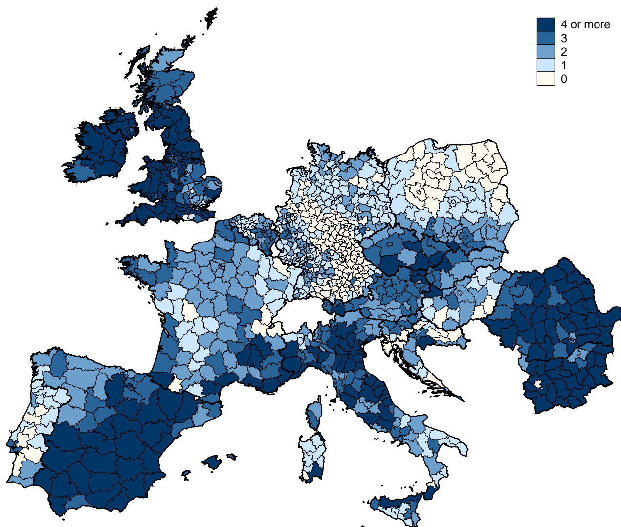
Figure 1: Flood map (2007-2018)
