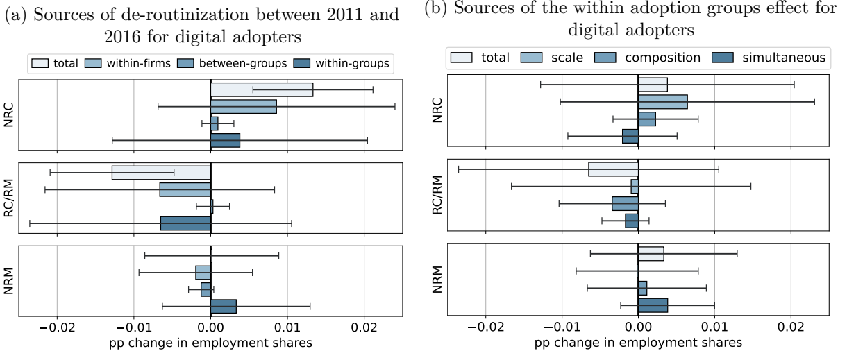
Figure D.2: Contribution of digital adopters to aggregate de-routinization
