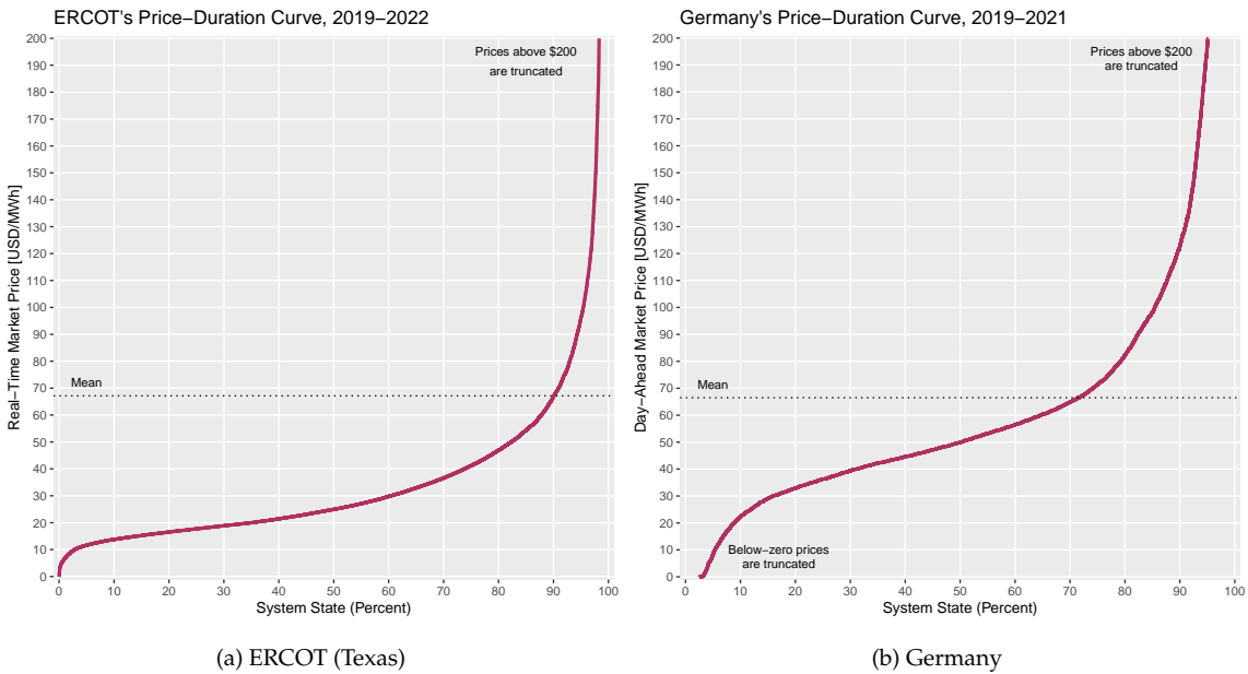
Figure A.2: Price-Duration Curves
