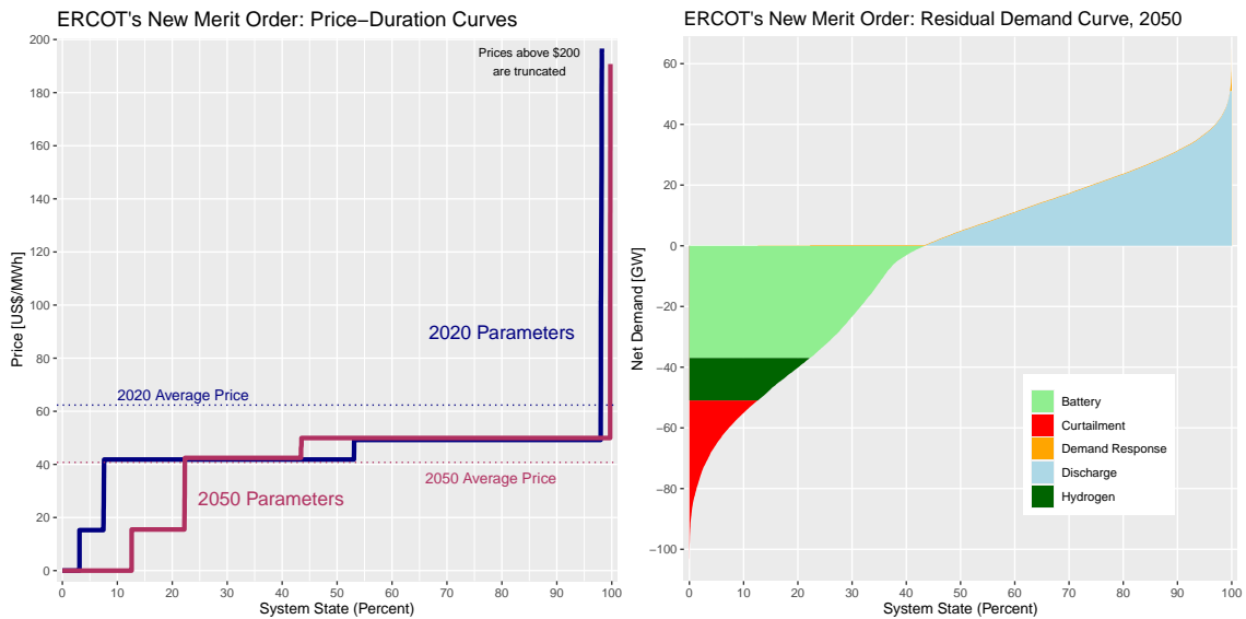
Figure 2: ERCOT's New Merit Order
