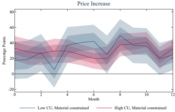
FIGURE 7: Price and production increases conditional on capacity utilization with and without material constraint
