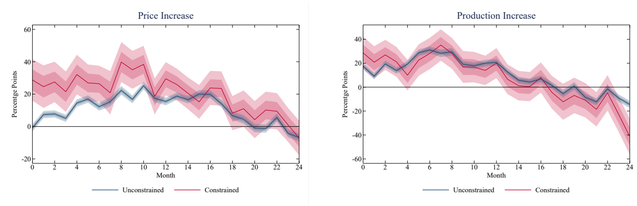
FIGURE E.18: Price and production increases conditional on material constraints: Long horizon
