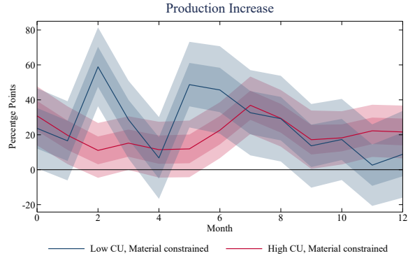
FIGURE 7: Price and production increases conditional on capacity utilization with and without material constraint
