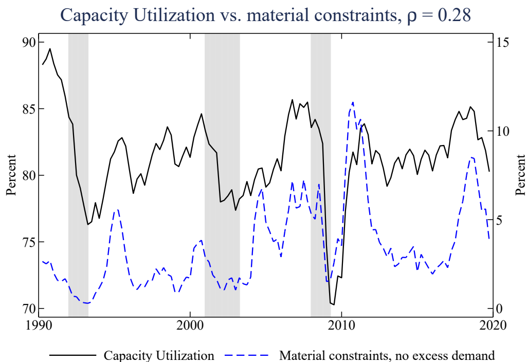
FIGURE E.10: Capacity utilization and material constraints without excess demand over the business cycle
