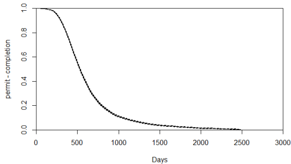
Figure 2: Kaplan-Meier plots
