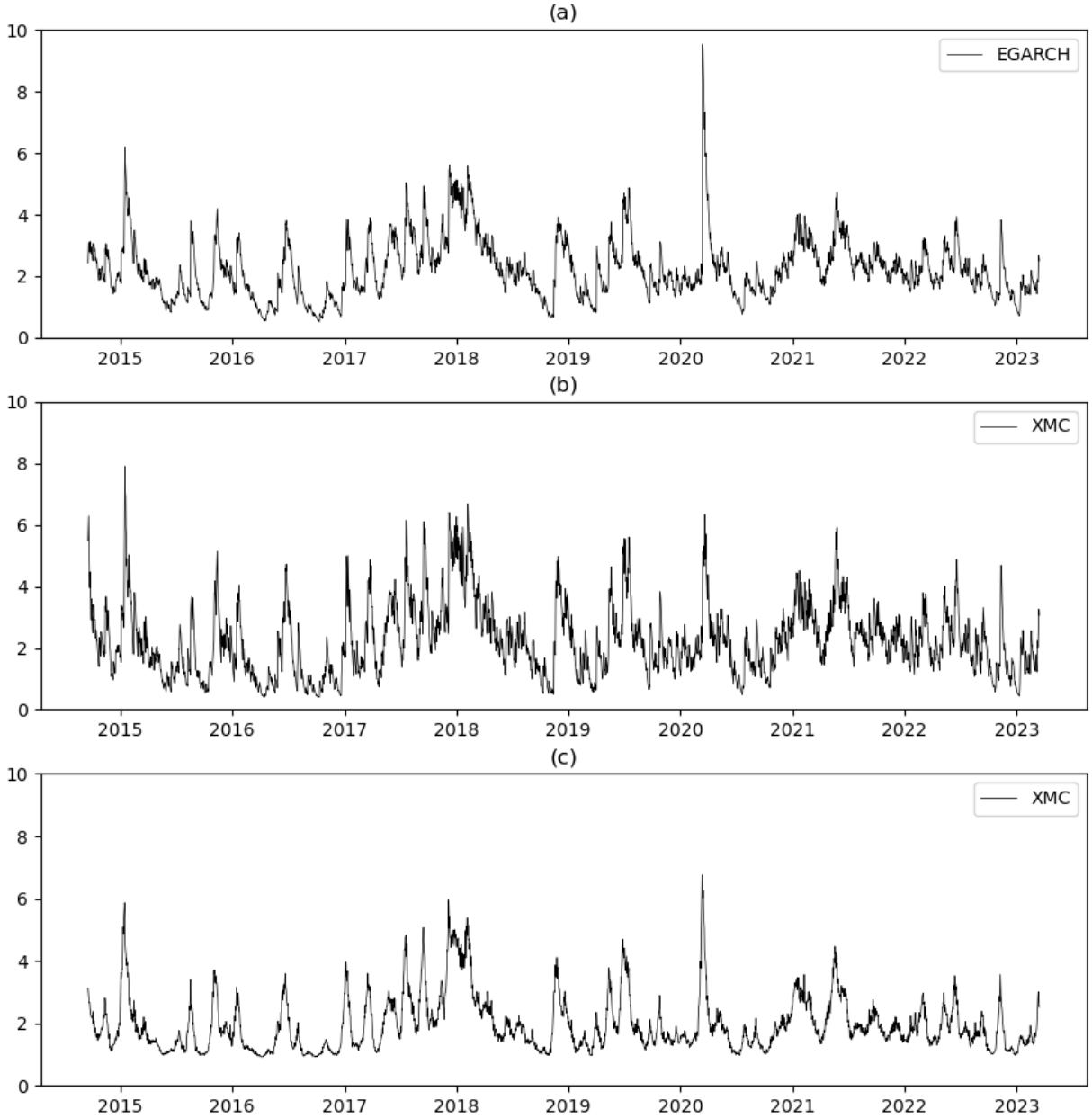
Figure 6: Estimated Bitcoin volatility \sigma_t = \exp(x_t/2) for the EGARCH-ST and GB-XMC filters: (a) filtered EGARCH volatility \exp(\hat{z}_t/2) based on the corresponding filter for z_t in (9); (b) XMC 1-period forecasts \mathbb{E}[\sigma_t|y_{1:t-1}] ( N = 10^6 ); (c) XMC smoothed volatilities \mathbb{E}[\sigma_t|y_{1:T}] ( N = 10^5 ).
