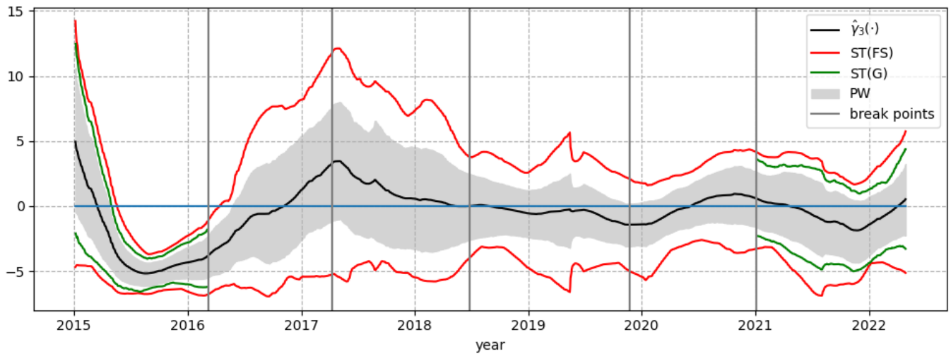
Figure 14: Estimated curve of \hat{\gamma}_3(\cdot) (black line) and resulting 95%-level confidence intervals (grey, labeled as PW) and bands using the SWB for Model (B.1), see Figure 3 for further information.
