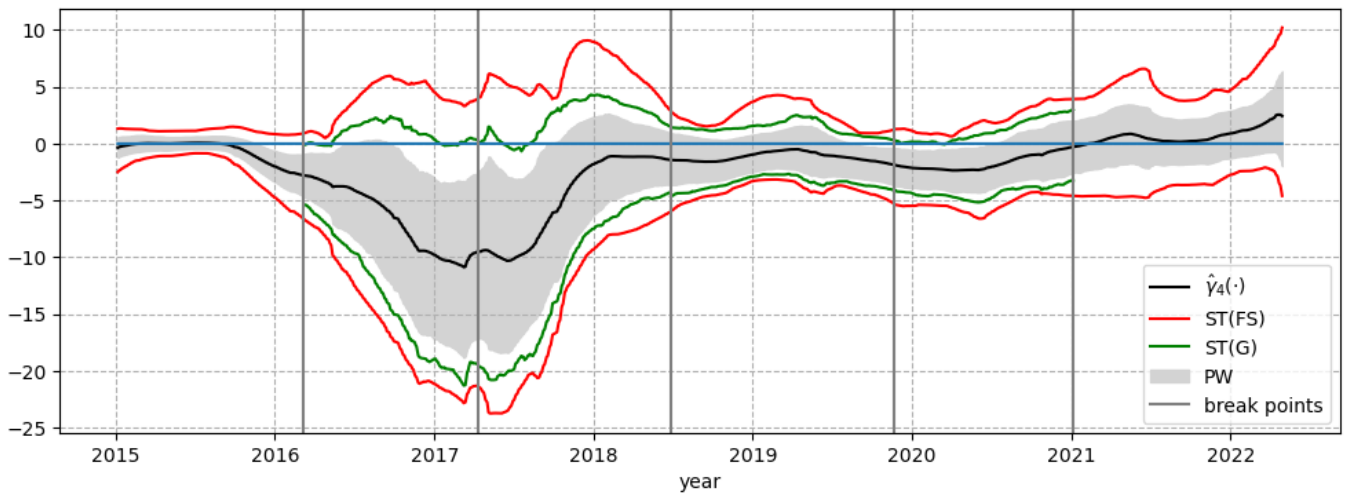
Figure 11: Estimated curve of \hat{\gamma}_4(\cdot) (black line) and resulting 95%-level confidence intervals (grey, labeled as PW) and bands using the SWB for Model (5.3), see Figure 5 for further information..
