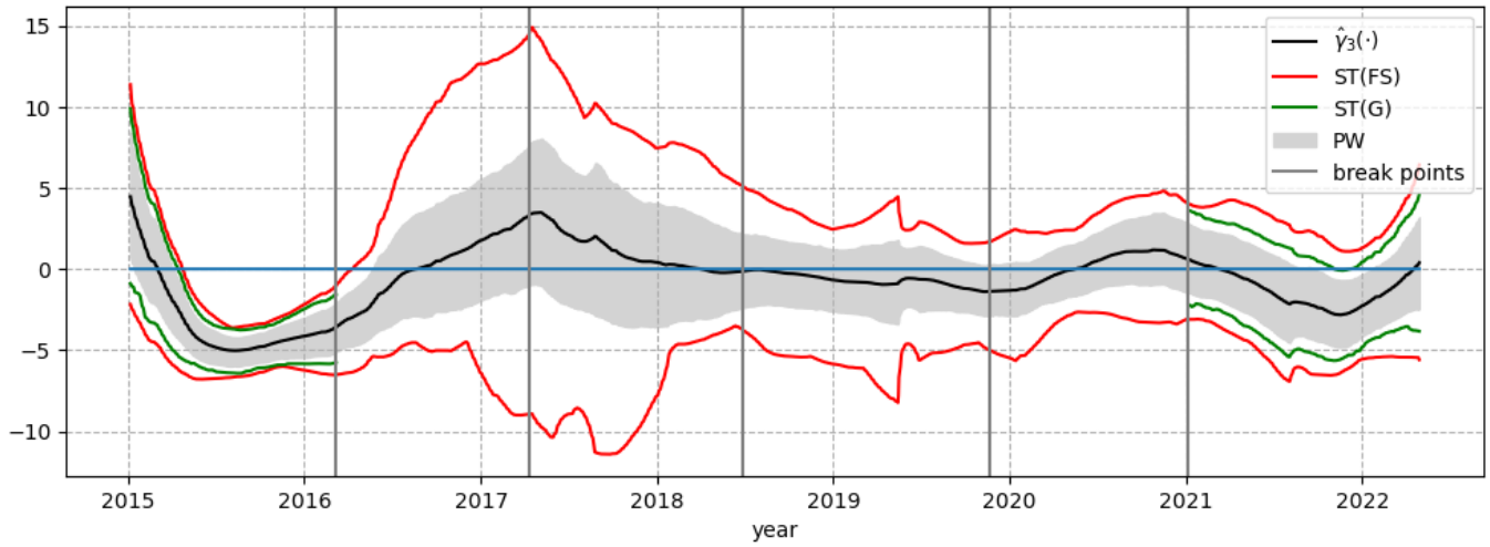
Figure 10: Estimated curve of \hat{\gamma}_3(\cdot) (black line) and resulting 95%-level confidence intervals (grey, labeled as PW) and bands using the SWB for Model (5.2), see Figure 3 for further information.
