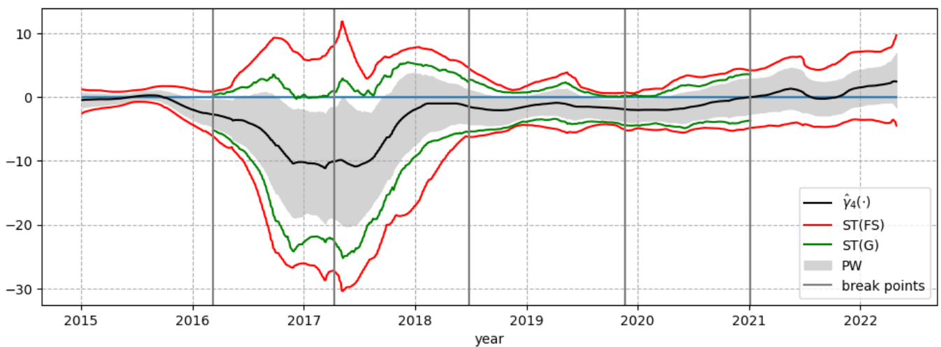
Figure 15: Estimated curve of \hat{\gamma}_4(\cdot) (black line) and resulting 95%-level confidence intervals (grey, labeled as PW) and bands using the SWB for Model (B.2), see Figure 5 for further information.
