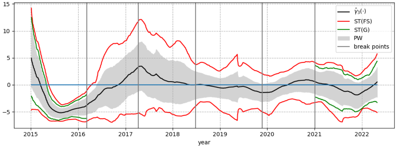
Figure 14: Estimated curve of \gamma_3(\cdot) (black line) and resulting 95%-level confidence intervals (grey, labeled as PW) and bands using the SWB for Model (B.1), see Figure 3 for further information.
