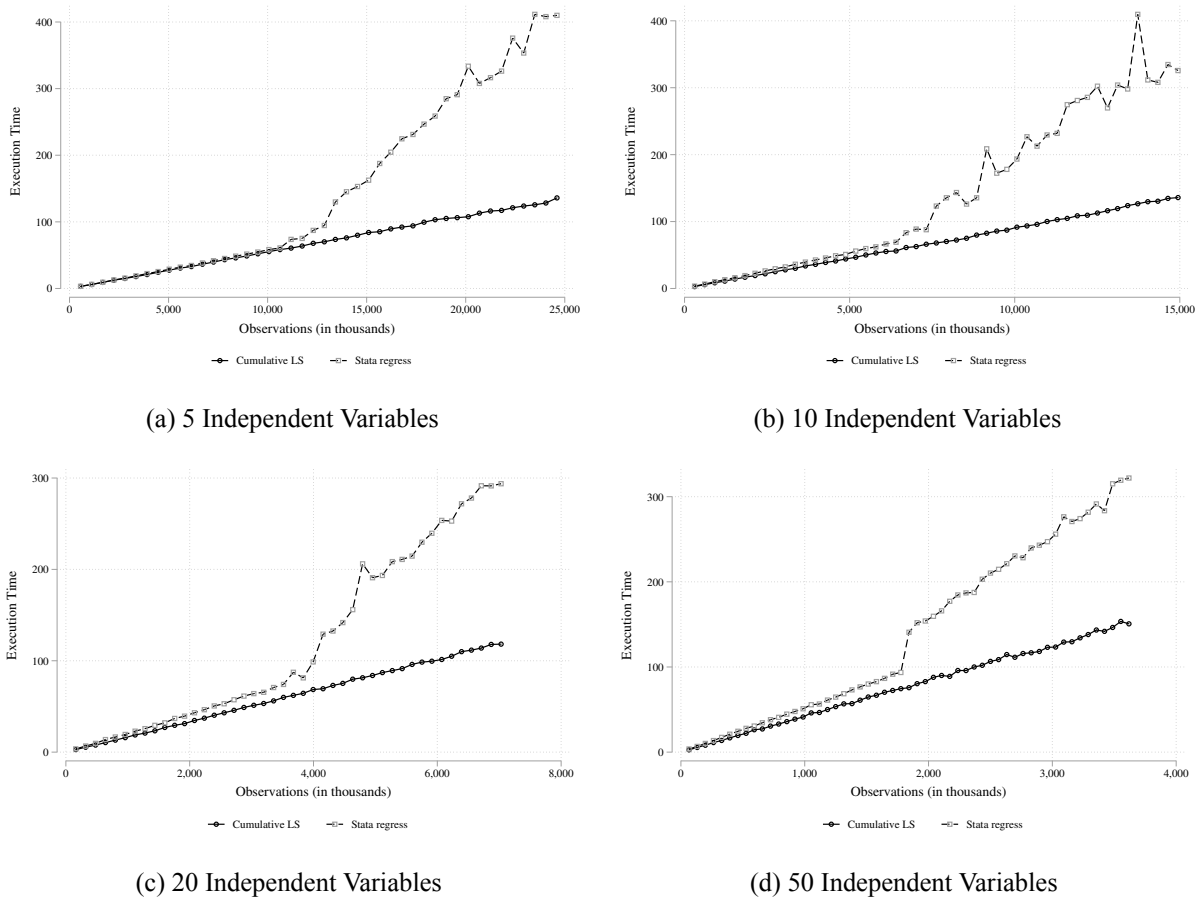
Figure 1: Sample size and execution time of commercial routine versus cumulative method
