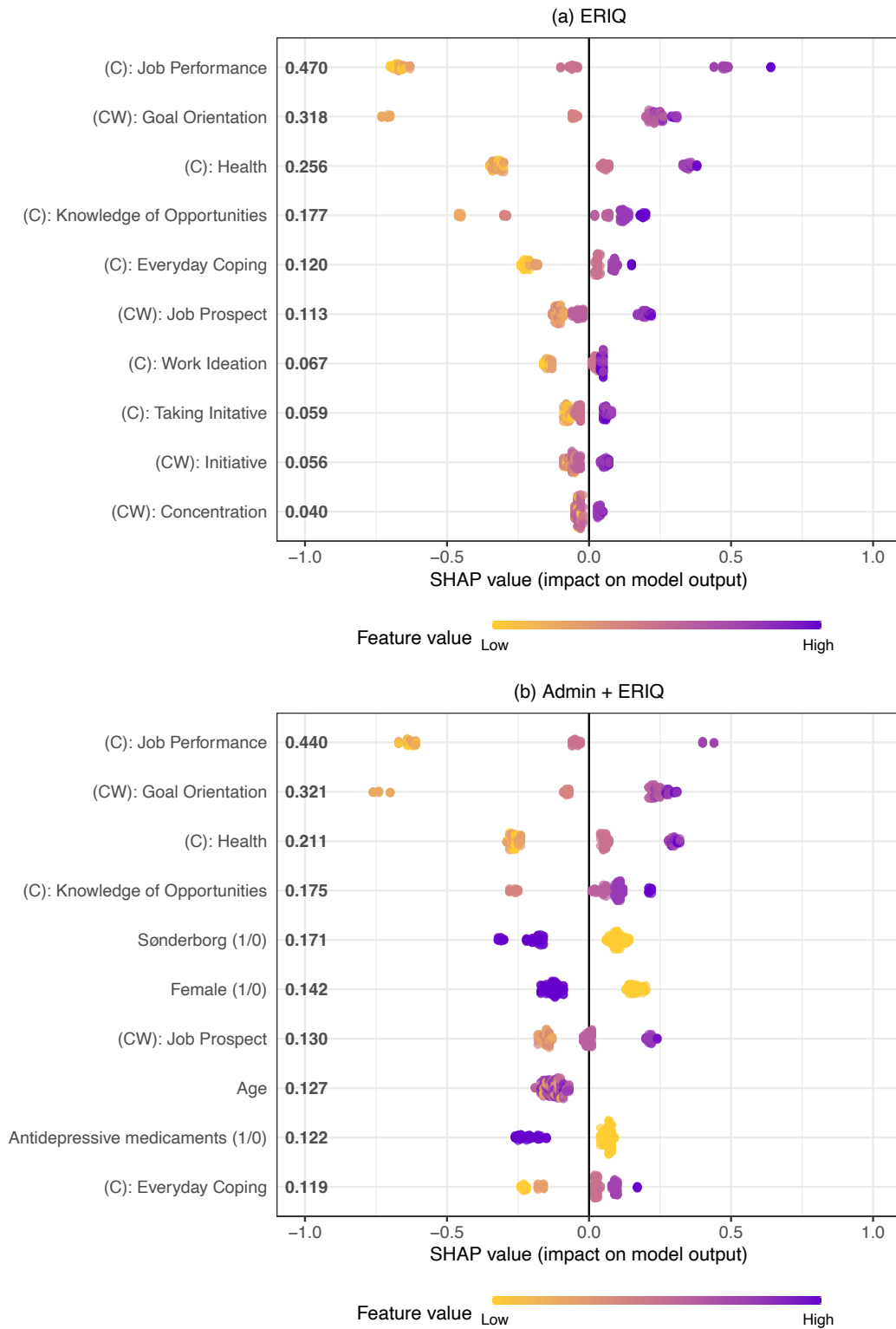
Figure 5: SHAP values for predicting job search
