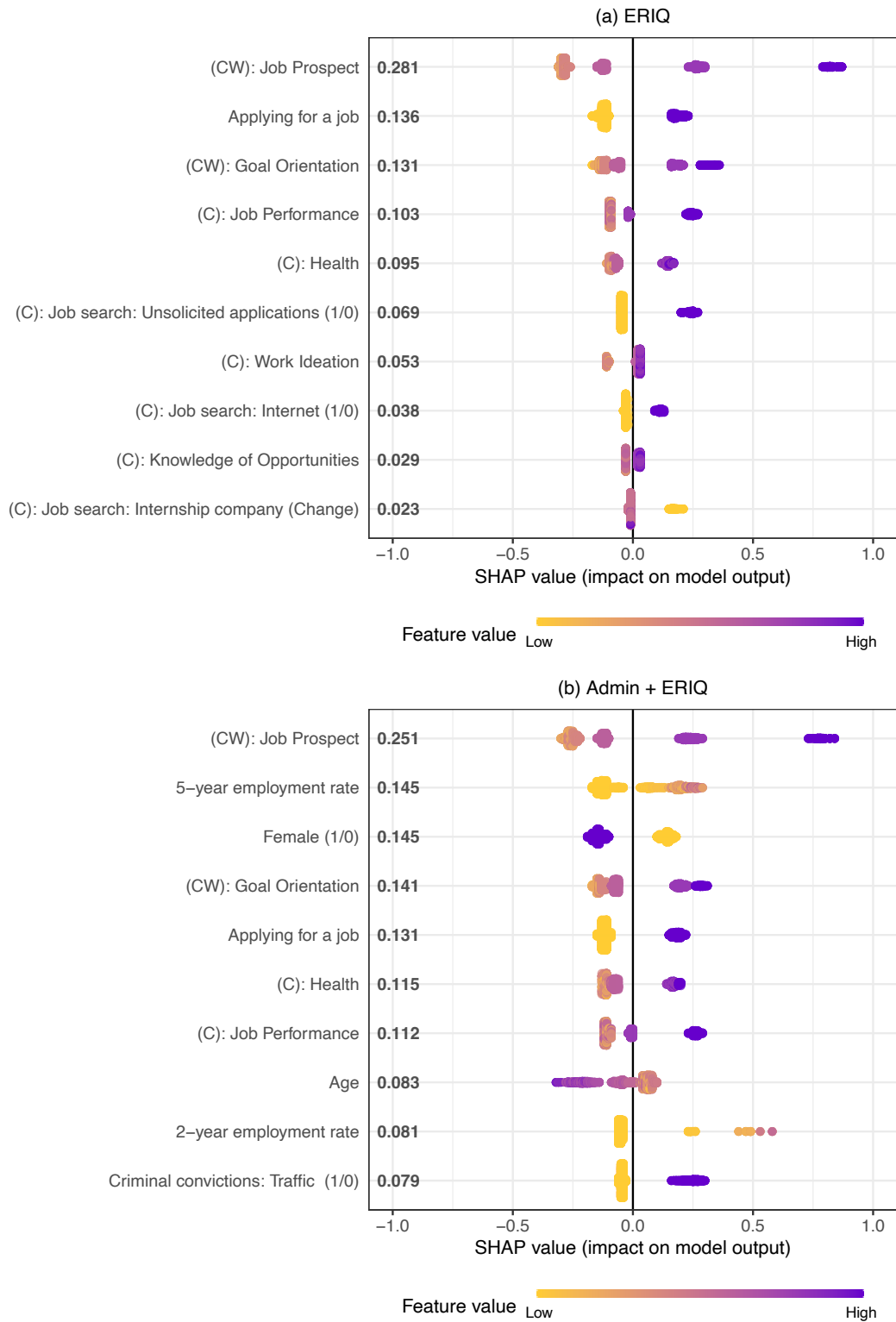
Figure 4: SHAP values for predicting the transition into employment
