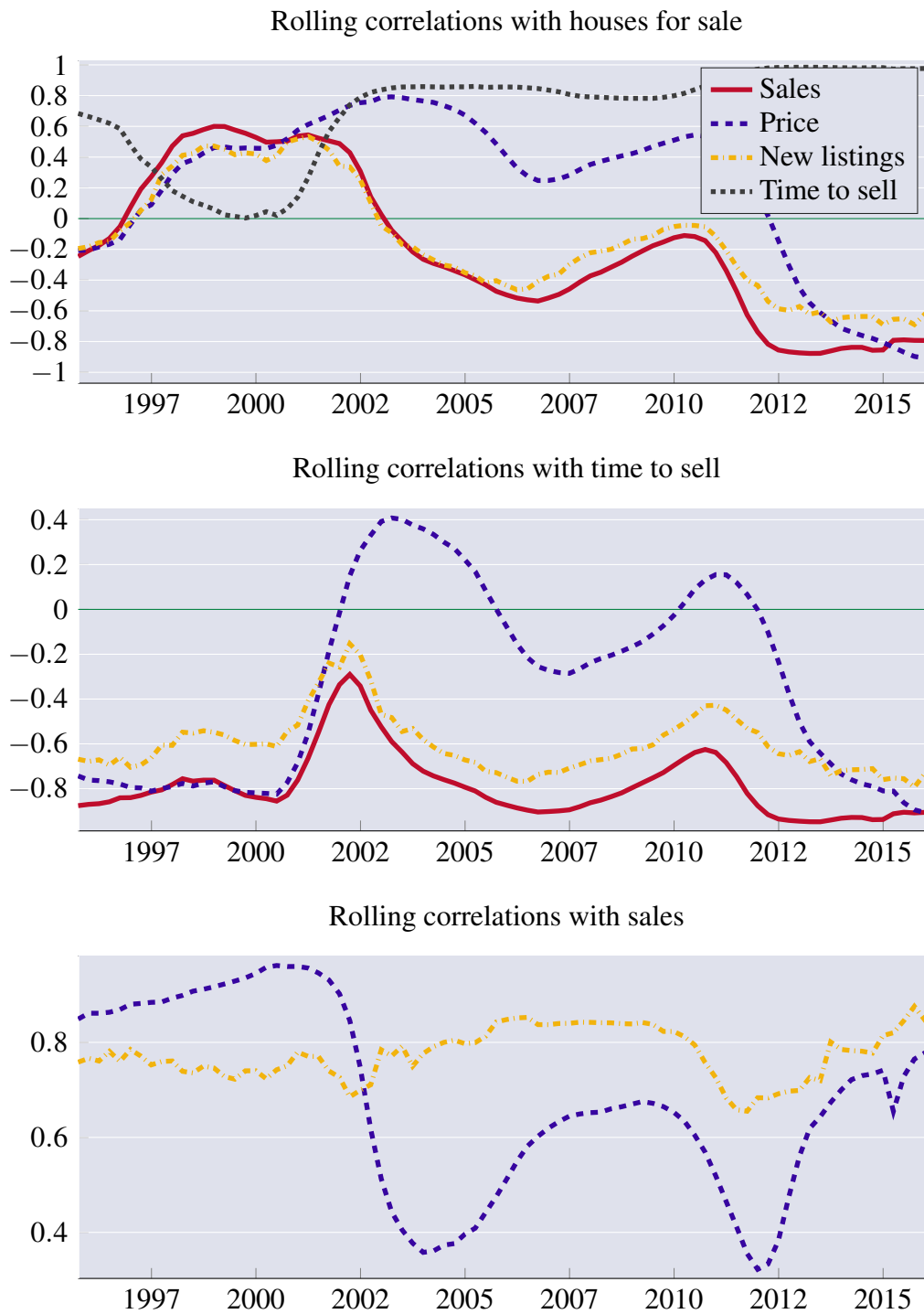
Figure A.2: Rolling correlations of housing-market variables without detrending
