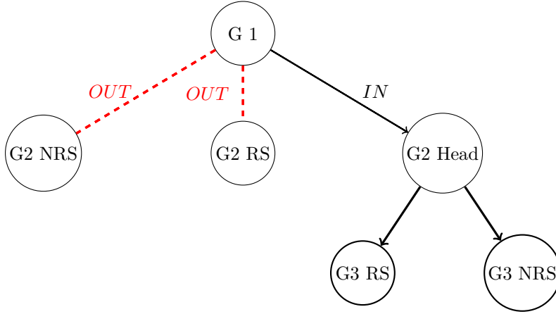
Figure 1: Generation tree
