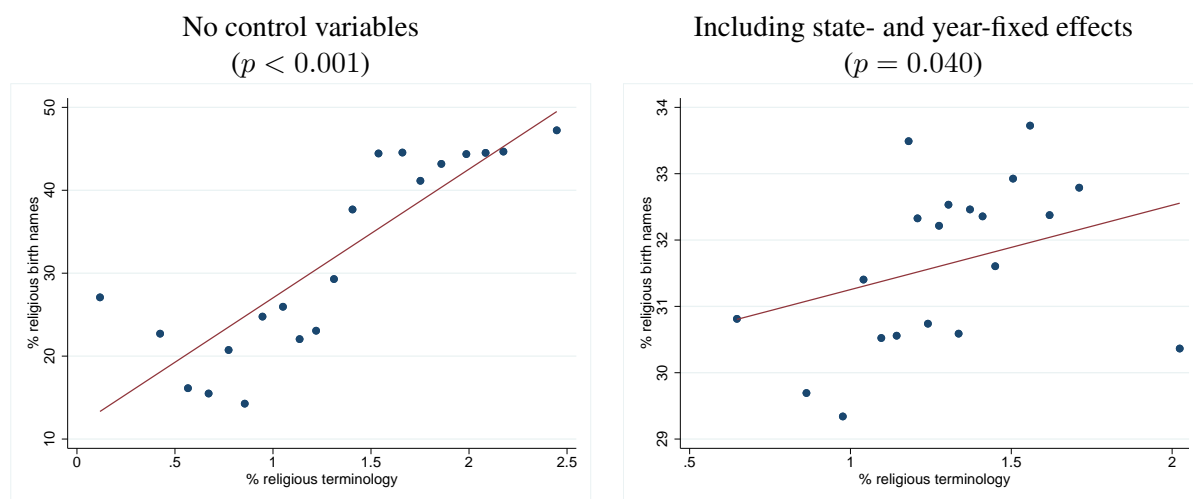
Figure 1: Binned scatterplots correlating the percentage of religious terminology on Google Ngram ( x -axis) with the percentage of religious birth names ( y -axis) between the years 1500 and 1714. Regressions include all 507 state-year observations for which both variables are available (i.e., from England, France, and Spain).
