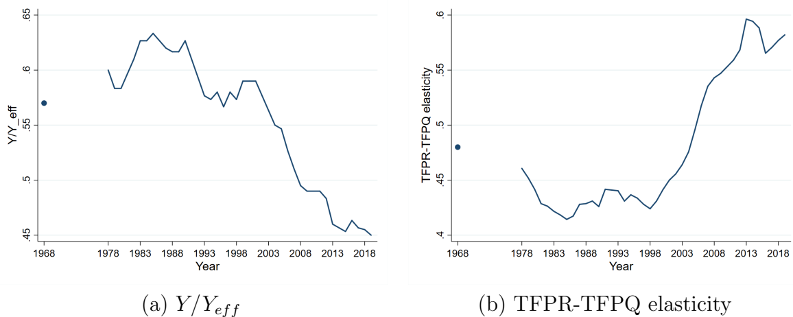
Figure 6: Allocative Efficiency
