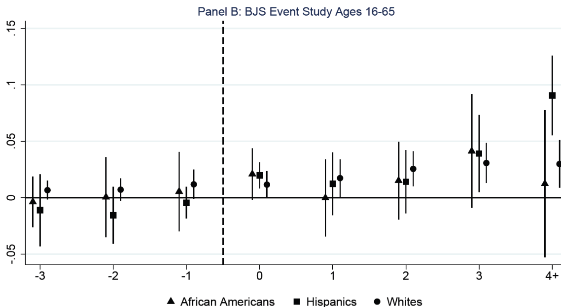
Figure 3. Event Studies of Changes in Underpayment For African Americans, Hispanics, and Whites Ages 16-65 Following Initial Statutory Minimum Wage Increases Using Various Event Study Estimators. This figure displays coefficients obtained from different event study estimators. Panel A displays results for African Americans, Hispanics, and non-Hispanic whites using the stacked event study estimator. Panel B displays results for African Americans, Hispanics, and non-Hispanic whites using the imputation estimator proposed by Borusyak, Jaravel, and Spiess (2021) (BJS). For all panels, the sample consists of all individuals ages 16-65 from the CPS MORG who are employed; paid by the hour; do not receive overtime, tips, or commissions; and do not have imputed wage rates. Estimates for statutory increases are plotted for “event” years ranging from 3 or 4 years before to 4 or 5 years after a state’s first statutory minimum wage increase occurred. The year of the initial increase is period 1 for the standard and stacked estimators in Panel A, and period 0 for the BJS estimator in Panel B. Error bars denote 95 percent confidence intervals around each estimated coefficient. Standard errors are clustered by state.
