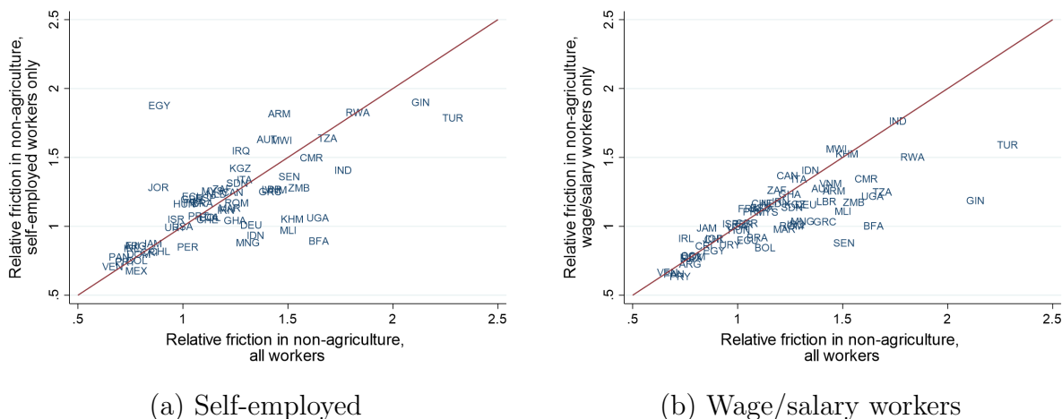
Figure C.1: Relative friction non-agriculture: self-employed and wage/salary workers vs all workers
