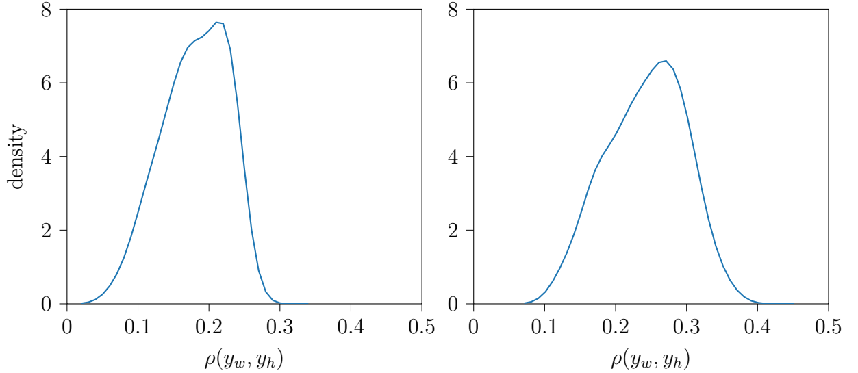
Figure 5: Estimated densities of \rho(y_w, y_h) 1976-1980
