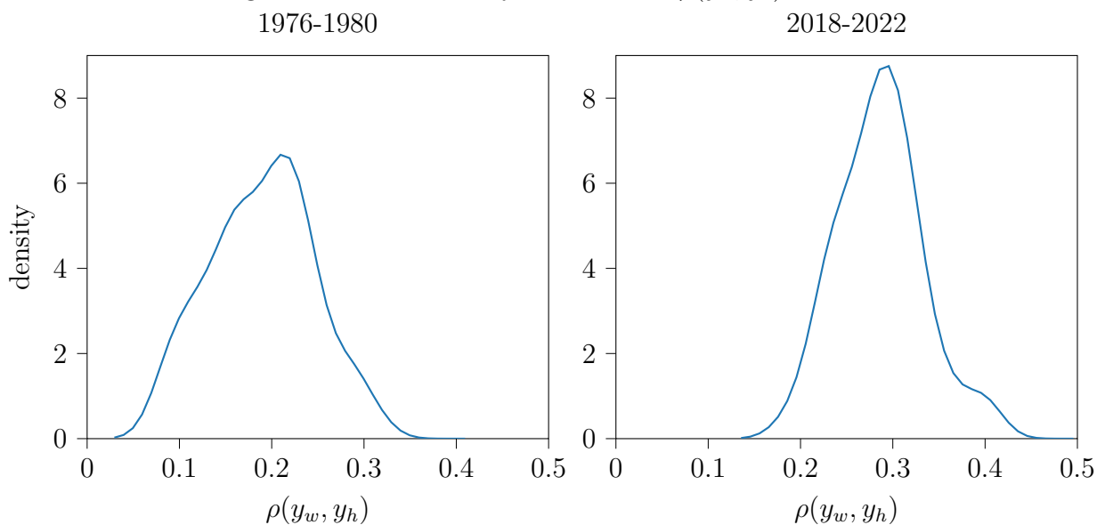
Figure 6: Kernel density estimates of \rho(y_w, y_h) .
