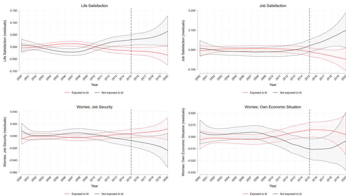
Figure 2: Exposure to AI and Workers' Well-being, 2000-2020 – Residualized Relationship
