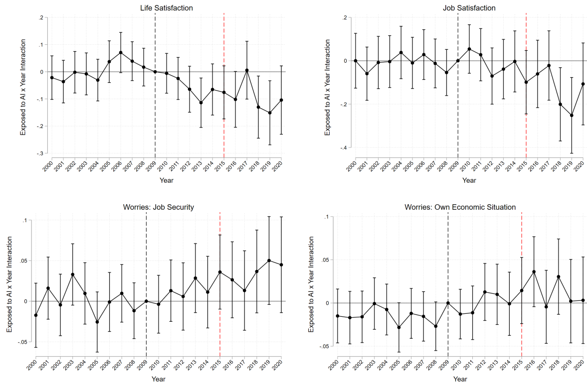
Figure 3: Exposure to AI and Workers' Well-being, 2000-2020 – Event Study Analysis
