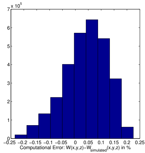
Figure A.1: Histogram of Computational Errors
