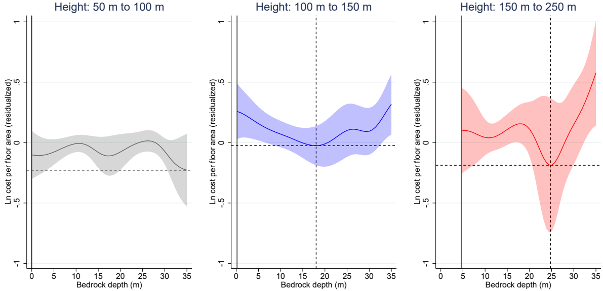
Figure A15: Construction cost as function of height and bedrock depths
