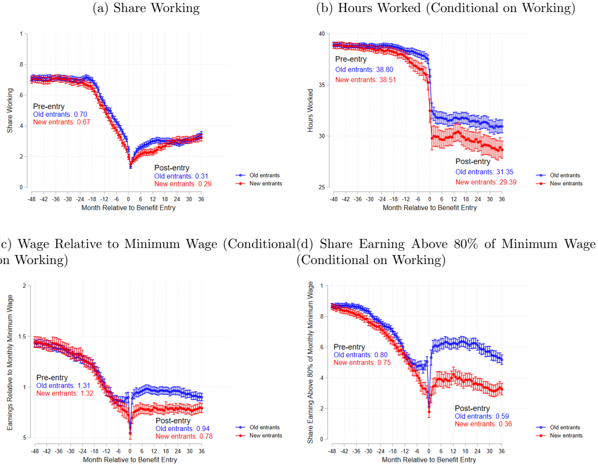
Appendix Figure A4: Reweighting
