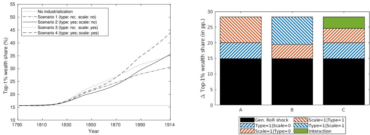
(a) Simulated trajectories of the top-1% share
