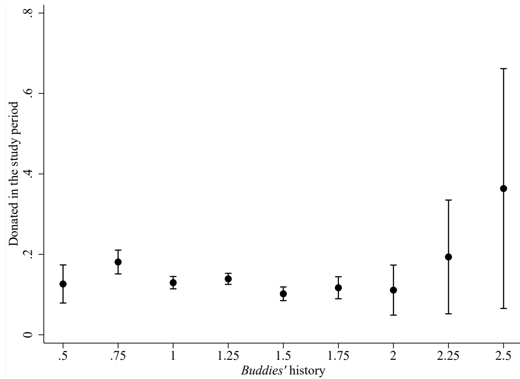
Figure C.4: Salient norm
