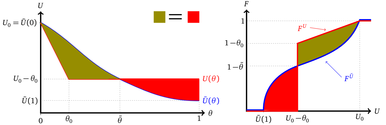
Figure 1: The left panel illustrates, given \tilde{U} and that \theta is uniformly distributed over [0, 1] , the construction of the cutoff contract U(\cdot) such that U_0 = \tilde{U}(0) and \int_0^1 U(\theta) d\theta = \int_0^1 \tilde{U}(\theta) d\theta . The right panel shows the associated probability distributions F^U and F^{\tilde{U}} of U and \tilde{U} in utility space. F^{\tilde{U}} is a mean preserving spread of F^U .
