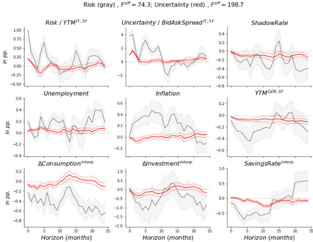
FIGURE 7: IMPULSE RESPONSE FUNCTIONS
