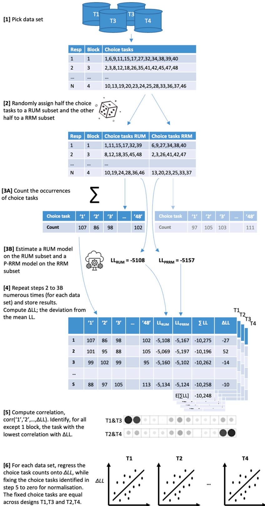
Fig. 2. Procedure to investigate decision rule heterogeneity.
