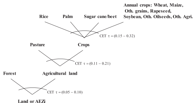
Fig. A.1. Nesting of constant elasticity of transformation function in the DART-BIOFISH model.
