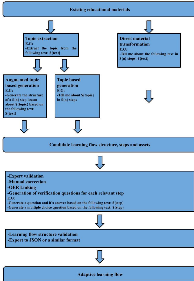
Figure no. 3 - Detailed conversion process diagram
