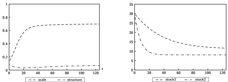
Figure 1: Optimal paths for scale and structure (left) and the two pollutant stocks (right) for the case \sigma_1 = \sigma_2 , \delta_1 < \delta_2 . Parameter values used for the numerical optimization are given in Appendix A.7.
