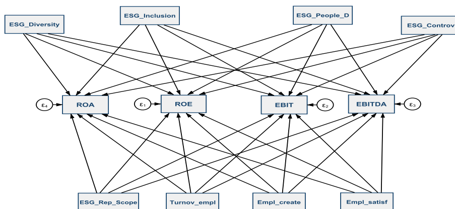
Figure no. 2. General pattern of SEM-2 designed to measure the interdependencies between the D&I coordinates and the financial performance of organizations
