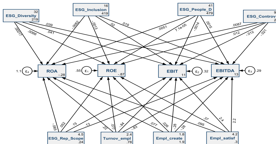
Figure no. 4. Results of SEM-2 to measure the interdependencies between the D&I pillars and the financial performance of organizations
