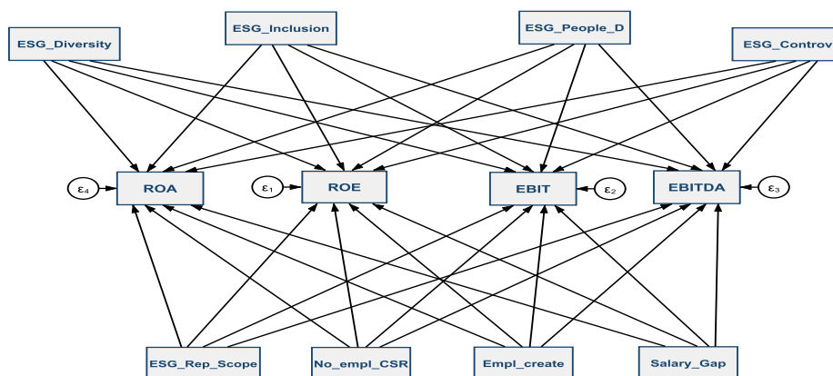
Figure no. 1. General pattern of SEM-1 designed to measure the interdependencies between the D&I coordinates and the financial performance of organizations
