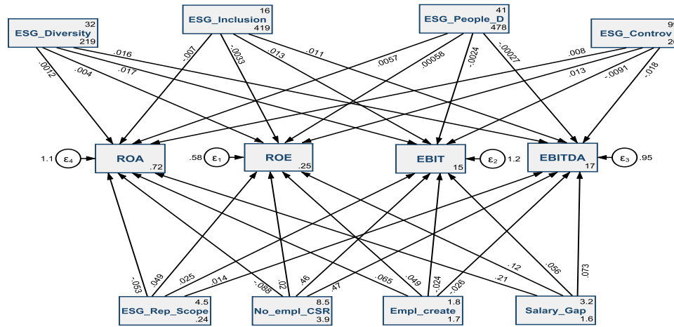
Figure no. 3. Results of SEM-1 designed to measure the interdependencies between the D&I pillars and the financial performance of organizations
