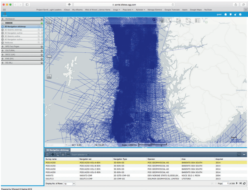
Figure 3.3 Map of seismic surveys on the southern part of the Norwegian continental shelf. The surveys (blue line) are so dense in large areas that they fill the map. Source: Reproduced by permission from the Norwegian Petroleum Directorate.
