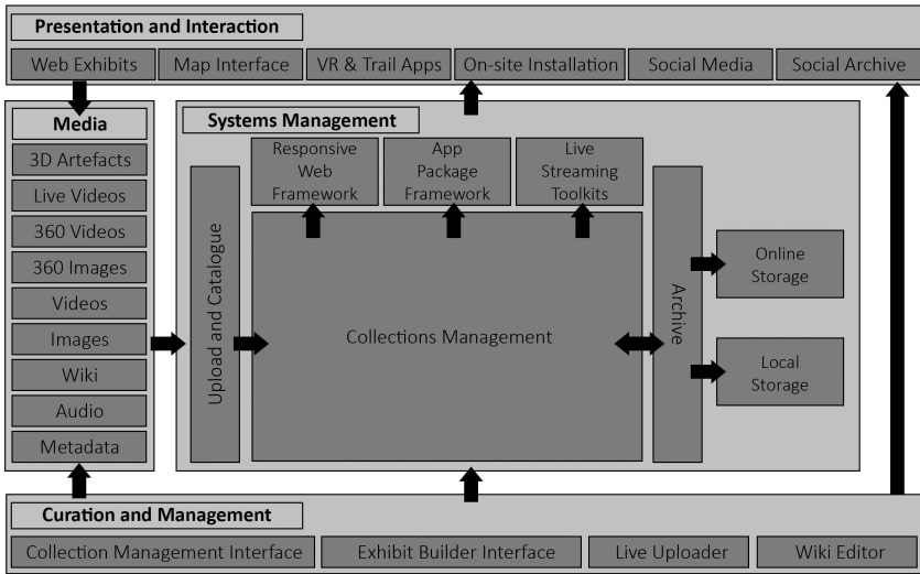
FIGURE 11.5 The architecture of a previously published VMI used for the VMCMM.
