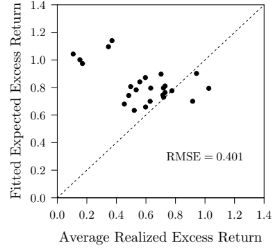
(b) FF3 Model + NMP
