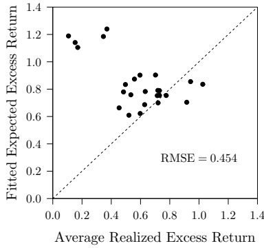
(c) FF3 Model + MOM
