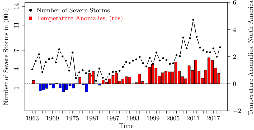
Figure 1: Temperature Anomalies and Number of Severe Thunderstorms
