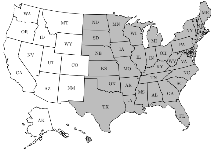
(a) NOAA Thunderstorm Risk Map
