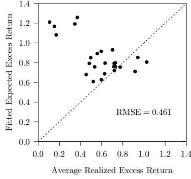
(a) FF3 Model
