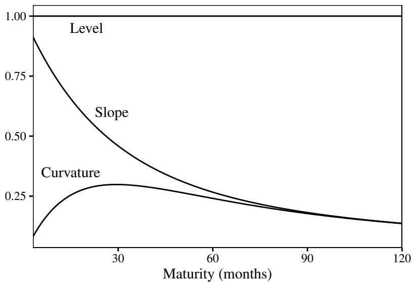
Figure 1: Nelson-Siegel factor loadings
