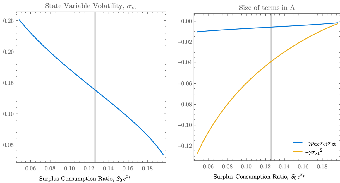
Figure 4: Terms related to TSU-Habit
