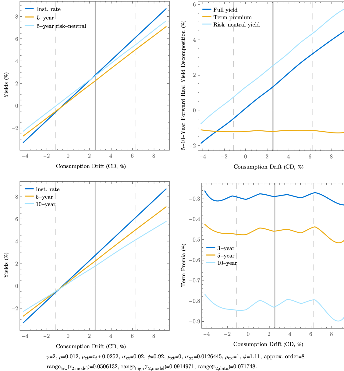
Figure 40: Time-varying consumption drift with recursive utility and high \rho_{cx} . See Figure 16 for more details about the plots.
