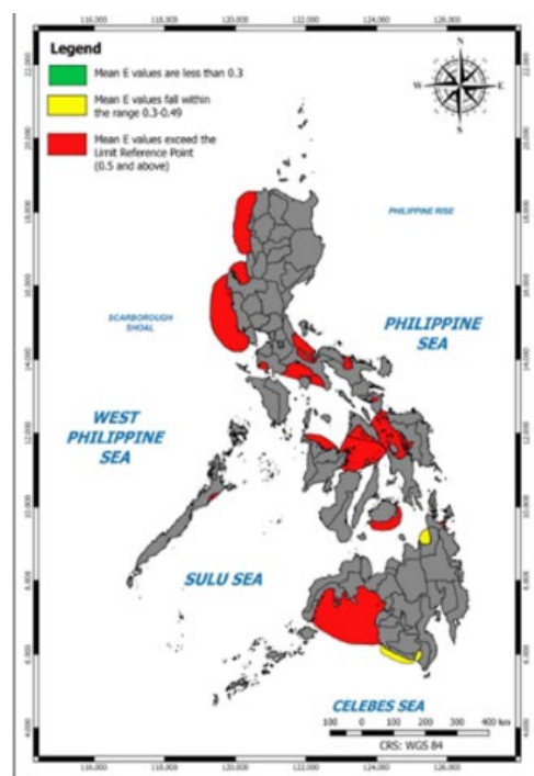
Figure 3.6. Status of Philippine Demersal Fish (based on Exploitation Values (E) using 2015 length frequency data and Limit Reference Point set at E=0.5)
