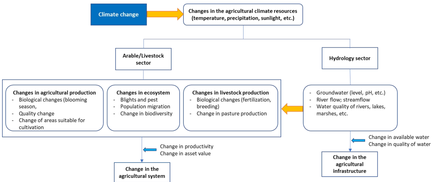
Figure 4.6. Climate Change Impact on the Agricultural Sector
