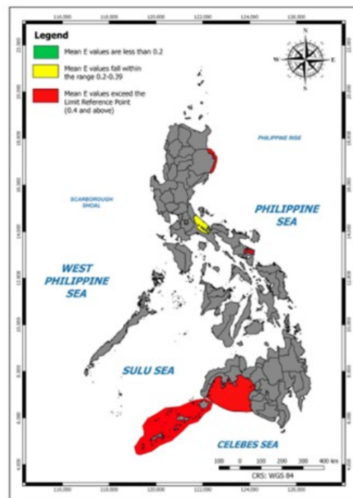
Figure 3.8. Status of Oceanic Tuna Fish (based on Exploitation Values (E) using 2015 length frequency data and Limit Reference Point set at E=0.4)
