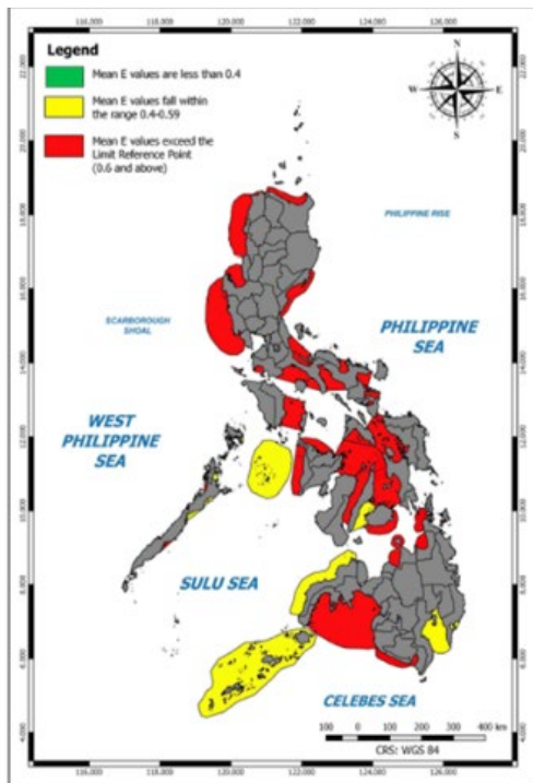
Figure 3.5. Status of Philippine Small Pelagic Fish (based on Exploitation Values (E) using 2015 length frequency data and Limit Reference Point set at E=0.6)
