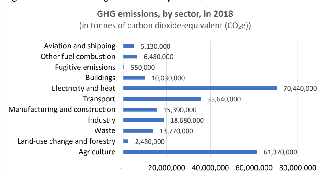
Figure 4.4: Greenhouse gas emissions by sector, in 2018
