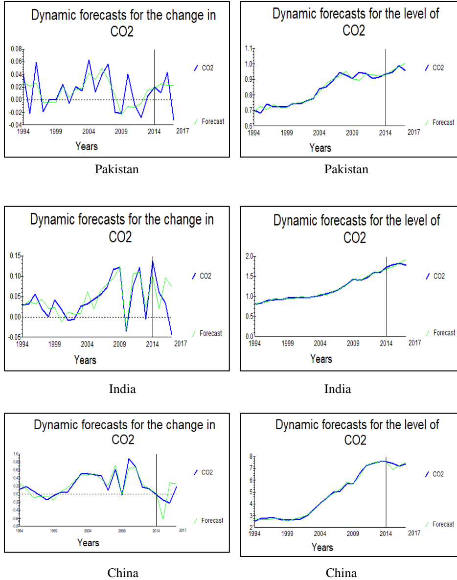
Figure 3: Plot of the dynamic forecasts for change & level of CO2 in PIC- Pakistan, India and China countries
