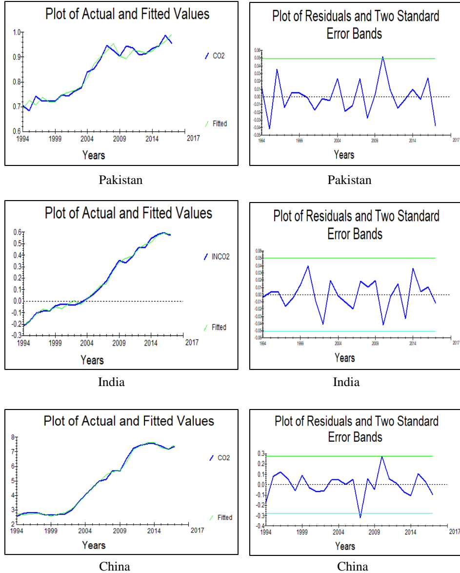
Figure 2: Plot of the in-sample actual values, fitted values and residual for Pakistan, India and China – PIC countries
