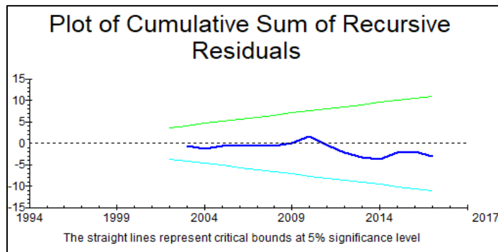
Figure 1: Plot of the CUSM for PIC – Pakistan, India and China
